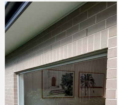
Brick Infill with Steel Lintel
